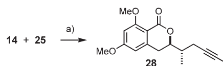
Scheme 3. a) \text{Me}_2\text{C}=\text{C}(\text{NMe}_2)(\text{Cl}) , 4-dimethylaminopyridine, \text{Et}_3\text{N} , 0^\circ\text{C} \rightarrow \text{RT} , quant.
